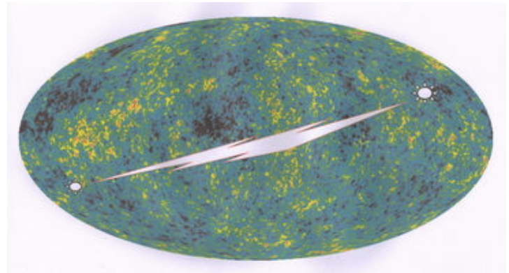
NON—LOCALITY UNIVERSE
