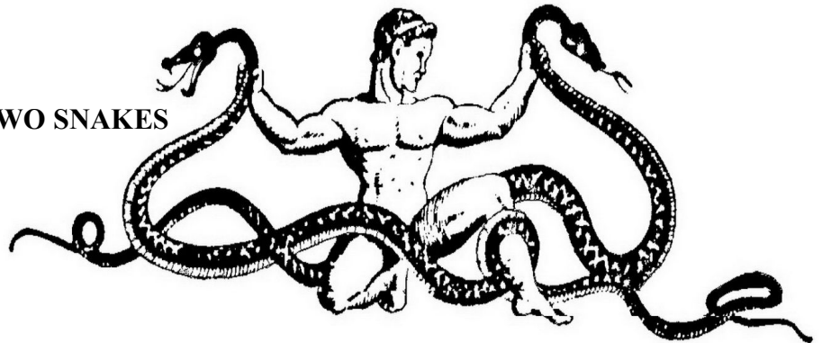
NON—LOCALITY UNIVERSE
